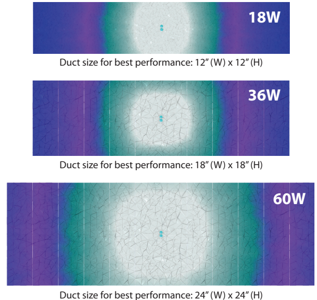
Figure 2: Fluence (UV-C intensity) field for Swordfish UV-C 18W, 36W & 60W lamps
