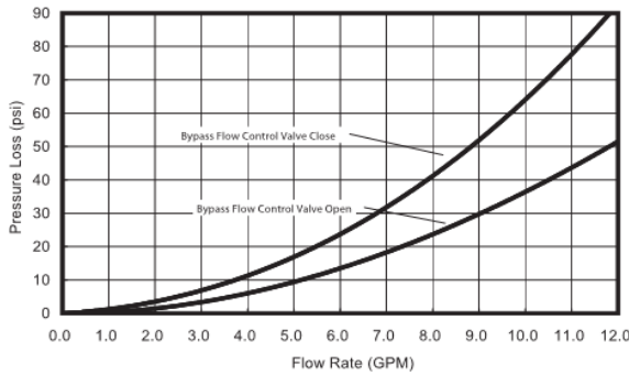
DHW Pressure Loss Curve
