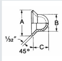
Copper Flare Seal Bonnets
