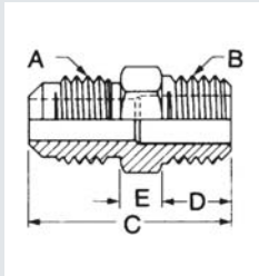
Half Union - Flare to NPTFE
