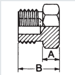
Brass Pipe Plug
