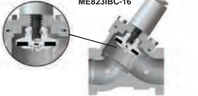
Integrated Back Check Feature
