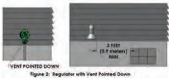
Figure 2: Regulator with Vent Pointed Down
