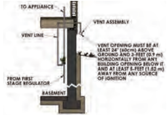
Figure 4: Basement Installation
