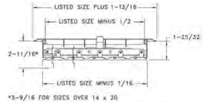
End View Showing Depth with Valve Open:
