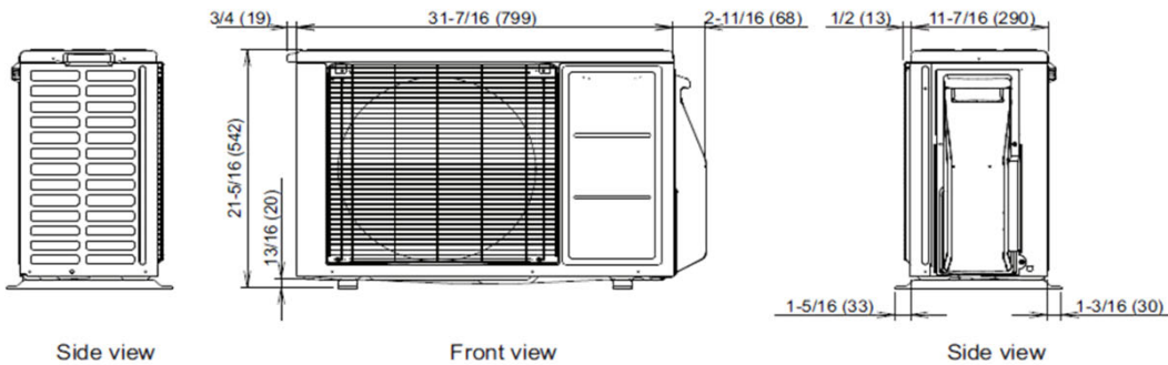
Side view
