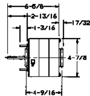
4 mounting bolts 3-1/2 dia. B.C. (Mounting Washers and Nuts Included)
